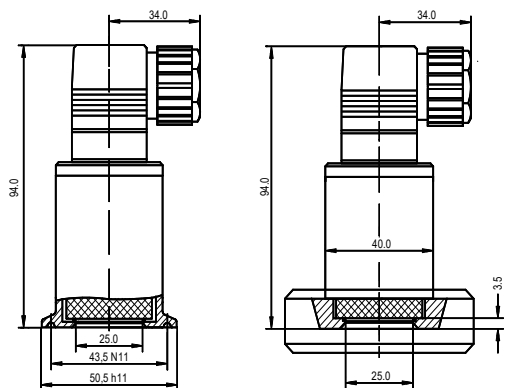
Clamp 1...1 1/2" DN 25...40
